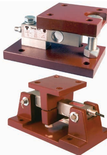
Low accuracy, general purpose weigh modules.
