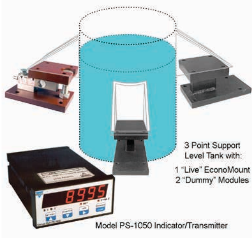
Simple level system with single weigh module support.
