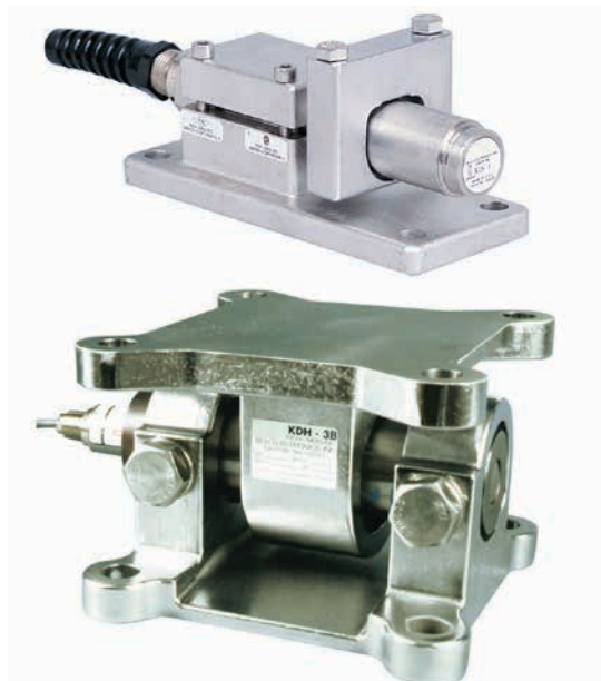
High accuracy, process weighing weigh modules.
